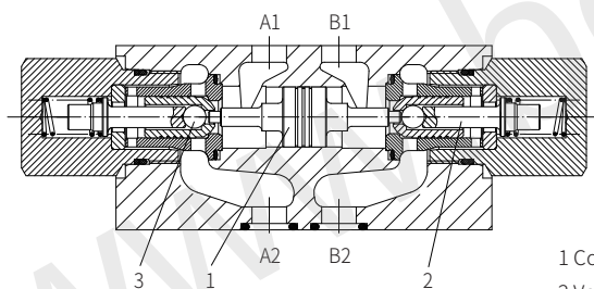
Model Z2S6...-6XJ/SO55 (with pre-opening)
