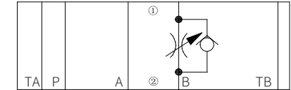
Model Z2FS10B-...-3XJ/...(meter-out control)
