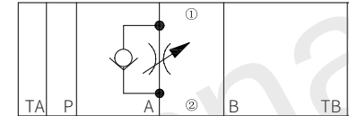
Model Z2FS10A-...-3XJ/...(meter-in control)
