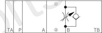
Model Z2FS10B-...-3XJ/...(meter-in control)
