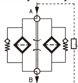
Differential pressure indicator
