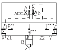
LFA.WEMB... size 40 to 50 Direction spool valve model: 4WE6D
