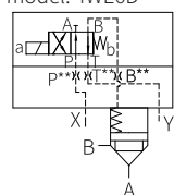
LFA.WEB... size 16 to 32 Direction spool valve model: 4WE6D
