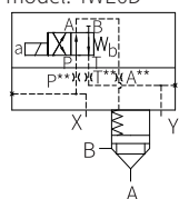
LFA.WEA... size 40 to 50 Direction spool valve model: 4WE6D
