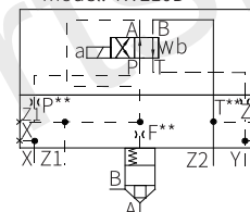
LFA.WEMA... Direction spool valve model: 4WE10D
