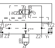
LFA.WEMA... size 40 to 50 Direction spool valve model: 4WE6D
