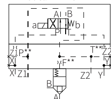
LFA.WEMB... Direction spool valve model: 4WE10D
