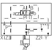
LFA.WEMB... size 16 to 32 Direction spool valve model: 4WE6D
