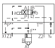
LFA.WEMA... size 16 to 32 Direction spool valve model: 4WE6D
