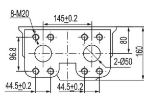
K向旋转 K Direction Rotation
