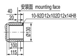
内花键 Female spline
