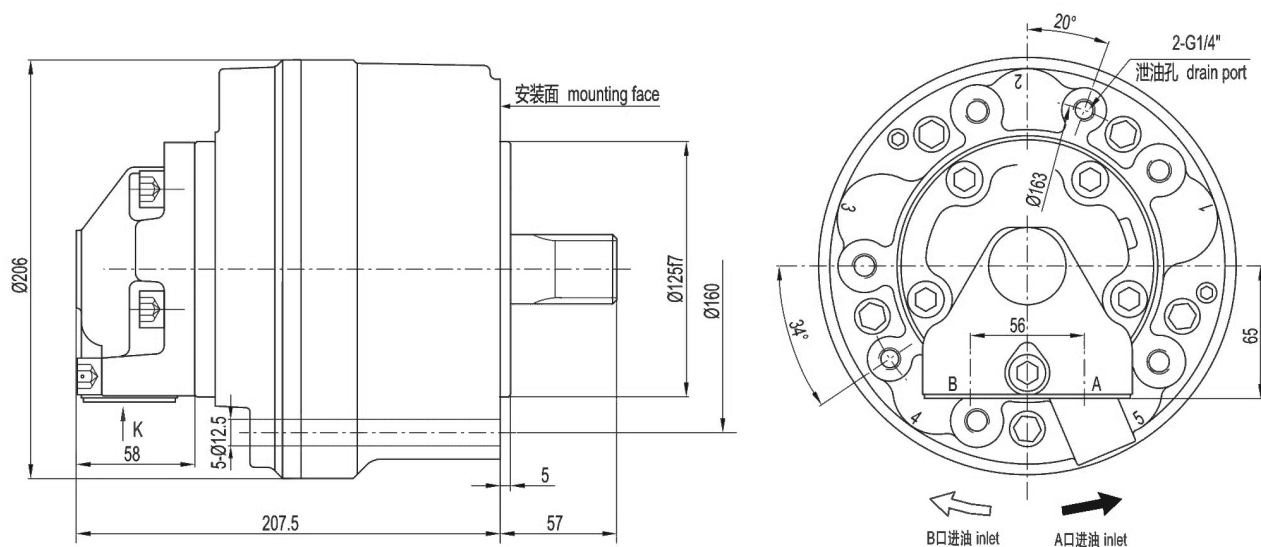
HGM05 外形及安装尺寸/ HGM05 Installation Dimensions
