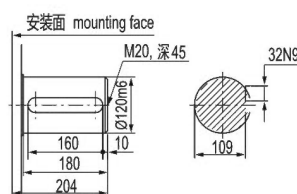
圆柱平键B Cylinder Flat Key B
