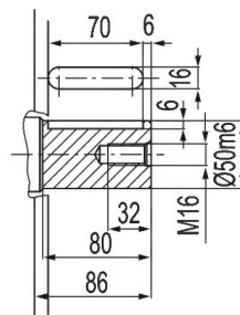
圆柱平键B Cylinder Flat Key B
