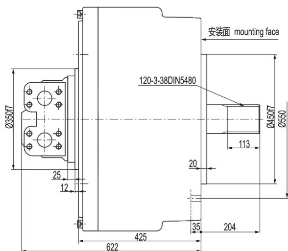
HGM9 外形及安装尺寸/HGM9 Installation Dimensions
