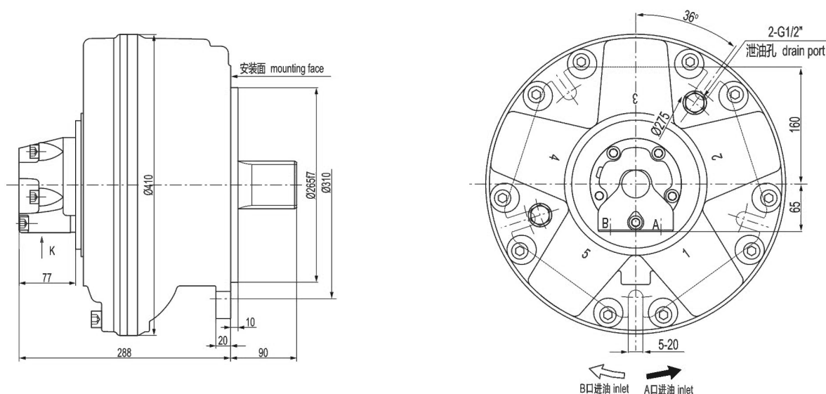
HGM4 外形及安装尺寸/HGM4 Installation Dimensions
