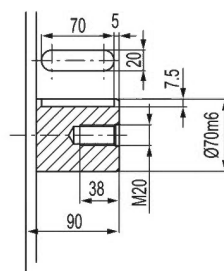
圆柱平键B Cylinder Flat Key B
