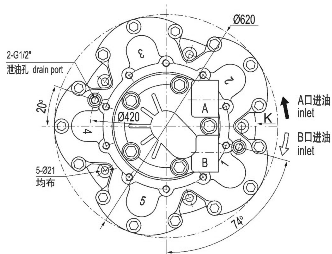
HGM7 外形及安装尺寸/HGM7 Installation Dimensions
