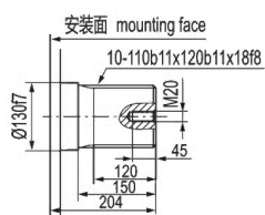
矩形外花键 Rectangular male spline
