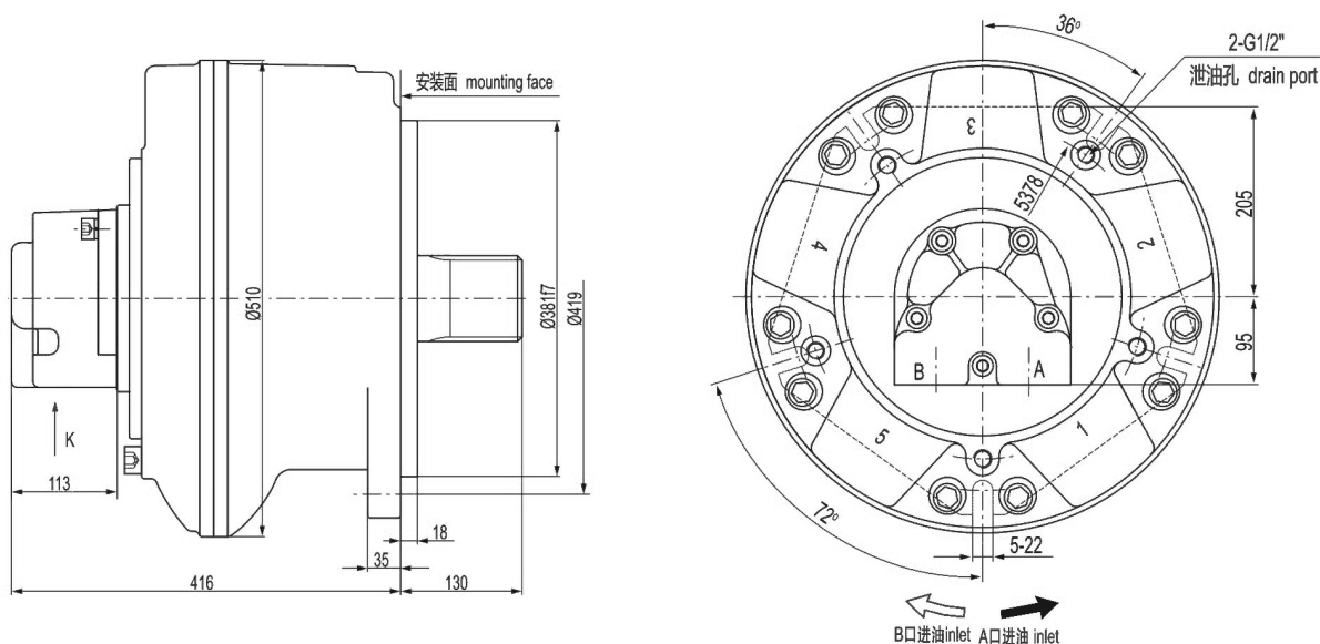
HGM6 外形及安装尺寸/HGM6 Installation Dimensions
