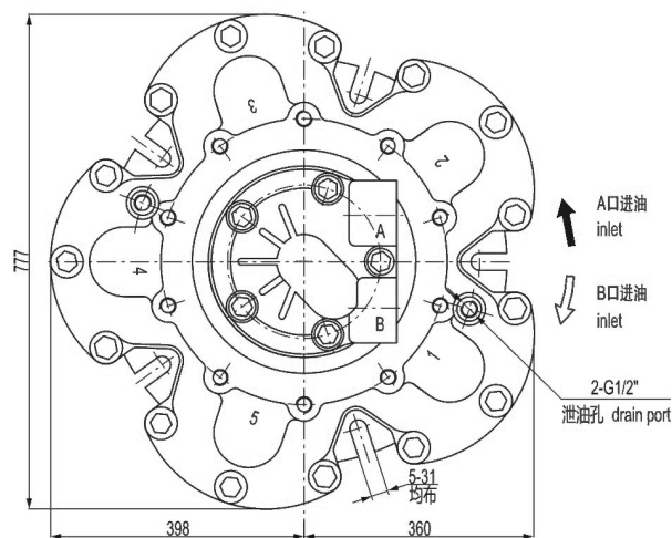
HGM9 外形及安装尺寸/HGM9 Installation Dimensions
