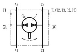
液压原理图/Hydraulic Schematic
