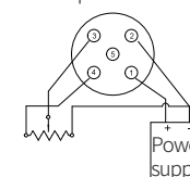
Connection example: Potentiometer input command
