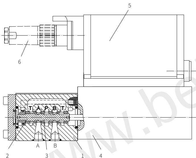
Model 4WRPEH6...-2XJ/
