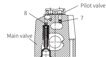
structure diagram of model WEH16...7XJ/ supply and drain
