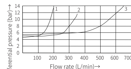
Model 4WEH16...-7X/.../P4.5
