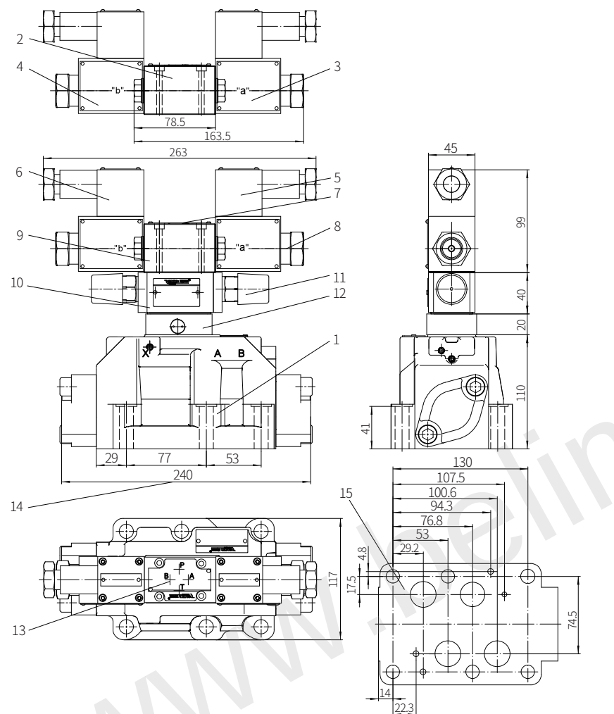
Model G-WEH22...-7XJ/...
