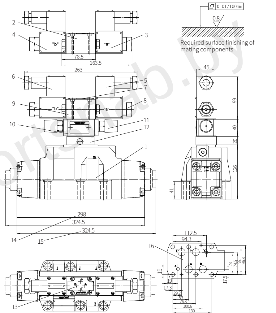
Model G-WEH25...-6XJ/...
