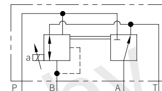
Model 3DREP...6B-2XJ/...E(detailed)
