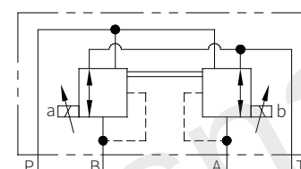
Model 3DREP...6C-2XJ/...E(detailed)
