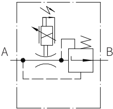
Proportional flow control valve (with integrated OBE)
