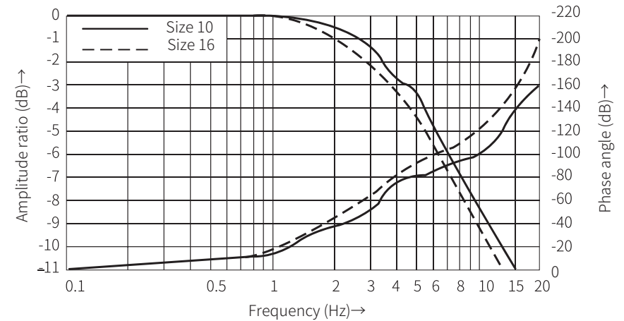
Frequency response characteristic curves
